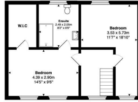
First Floor
